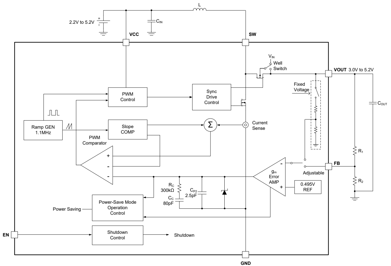
Figure 4. Block Diagram
