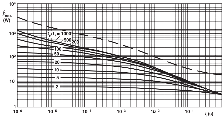
PR03 Pulse on a regular basis; maximum permissible peak pulse power ( P_{max} ) as a function of pulse duration ( t_i )
