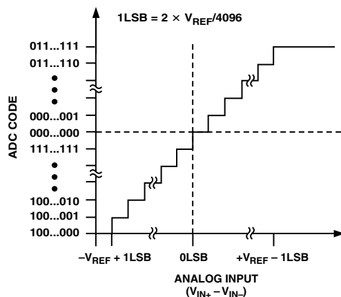
Figure 5. Ideal Transfer Characteristics
