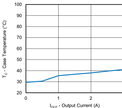
Fig. 34 - SiC474 Load Current vs. Case Temperature, V_{IN} = 48\text{ V} , V_{OUT} = 12\text{ V}
