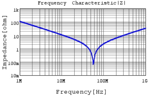
RCE5C2E152J1K1H03B |Z| DCOV, 25degC
