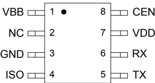
Figure 3. 33660 Pin Connections
