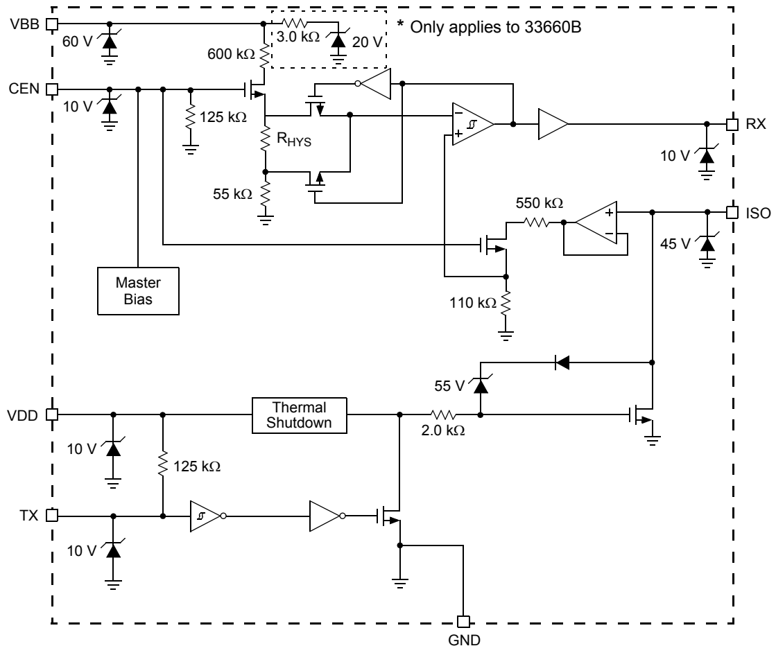
Figure 2. 33660 Simplified Internal Block Diagram
