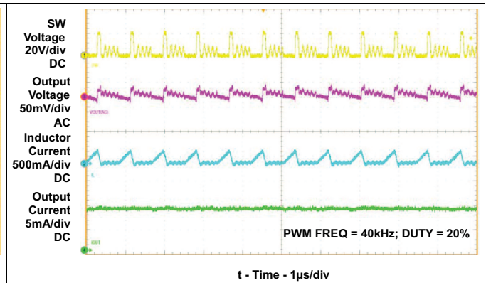
Figure 22. Switching Waveform
