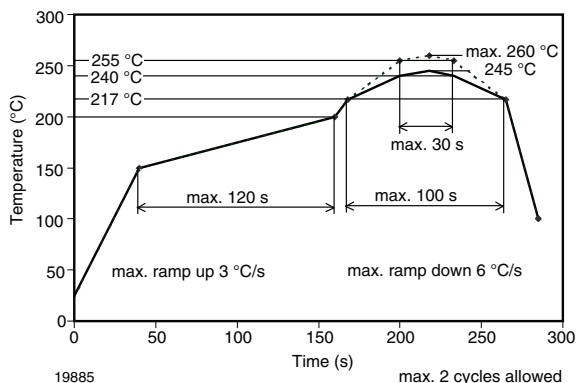
Fig. 9 - Vishay Lead (Pb)-free Reflow Soldering Profile (acc. to J-STD-020C)
