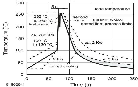
TTW Soldering (acc. to CECC00802)
