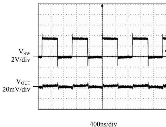
Figure 8. Light Load Operation ( V_{IN}=3.6V , V_{OUT}=1.8V , I_{OUT}=0mA )
