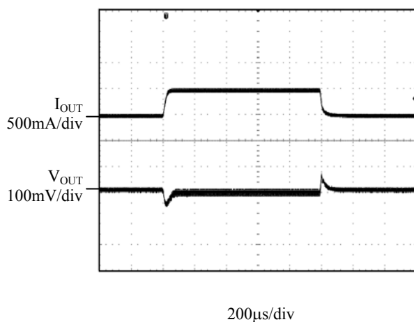
Figure 10. Load Transient ( V_{IN}=3.6V , V_{OUT}=1.8V , I_{OUT}=0mA to 500mA )
