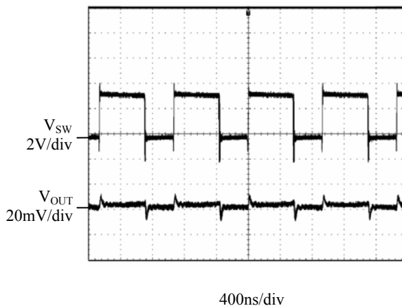
Figure 9. Heavy Load Operation ( V_{IN}=3.6V , V_{OUT}=1.8V , I_{OUT}=600mA )
