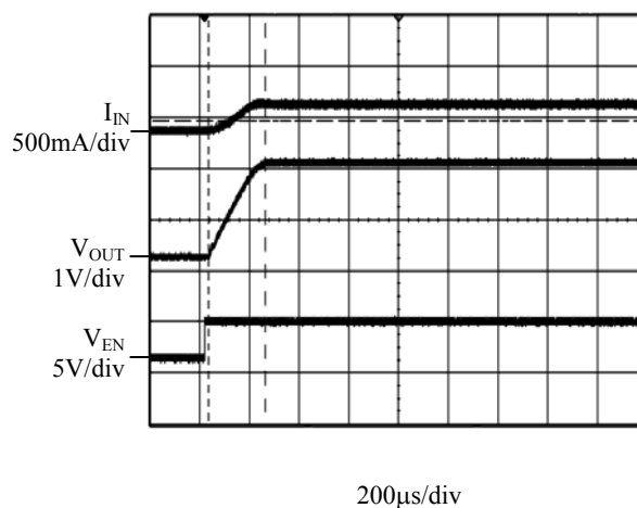
Figure 11. Start up from Shutdown ( V_{IN}=3.6V , V_{OUT}=1.8V , R_{LOAD}=4\Omega )
