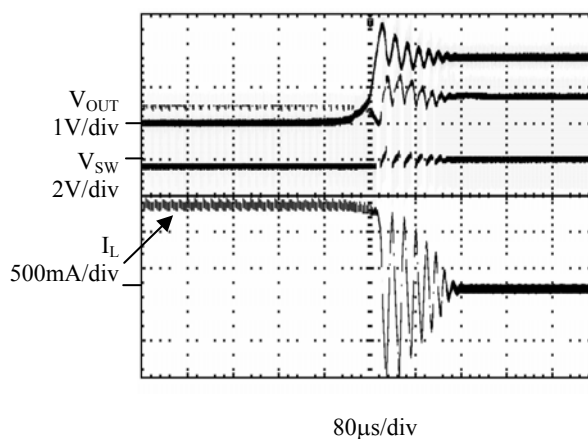
Figure 13. Short Circuit Recovery ( V_{IN}=3.6V , V_{OUT}=1.8V , no load)
