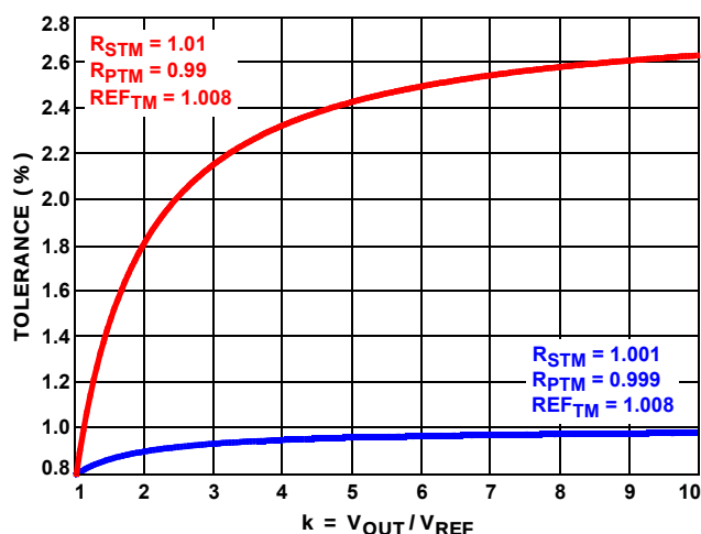
FIGURE 29. WORST CASE SYSTEM DC REGULATION TOLERANCE ( V_{REF} AT 0.8% ABOVE NOMINAL)
