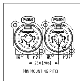
C TYPE LOW PROFILE MOUNTING PITCH
