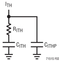
Figure 2. External Compensation Network
