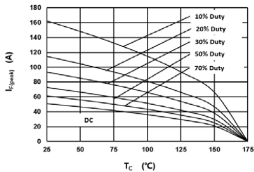
Fig 3: Current Derating
