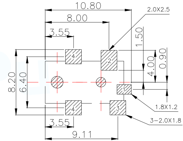
PCB.WELDING DRAWING (TOLERANCE:±0.05)
