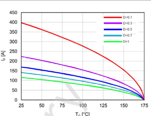
Figure 2. Current Derating
