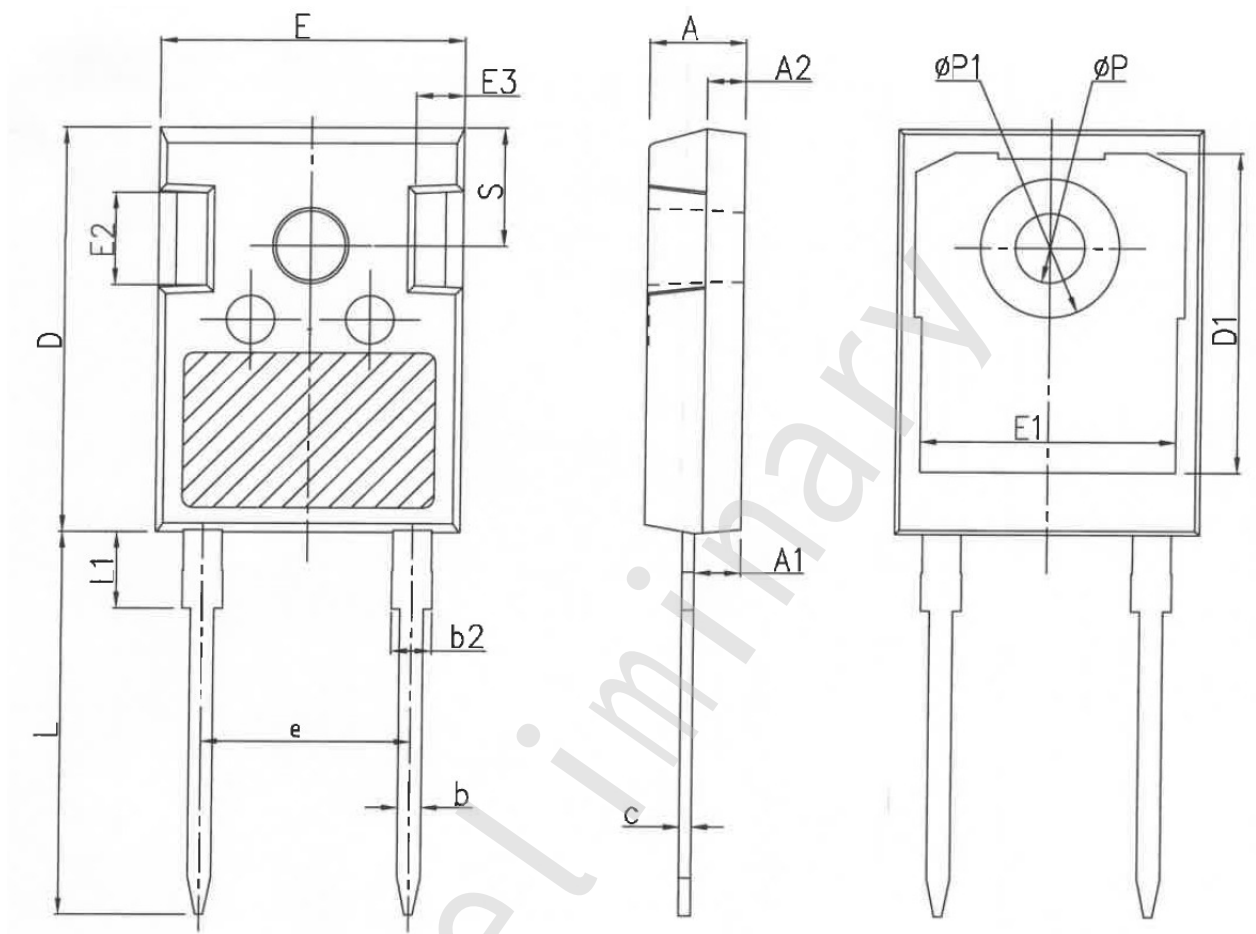
COMMON DIMENSIONS
