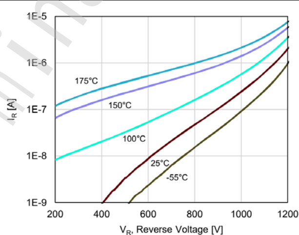
Figure 4. Reverse Characteristics
