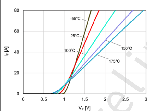
Figure 3. Forward Characteristics
