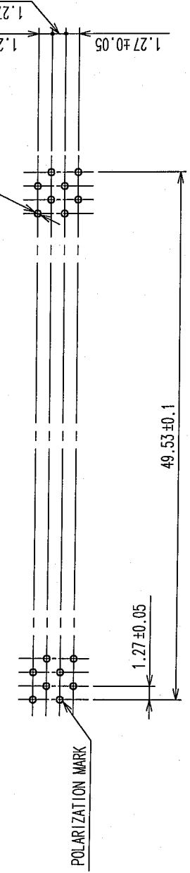
RECOMMENDED P.C.B. LAND PATTERN (MOUNT SIDE)
