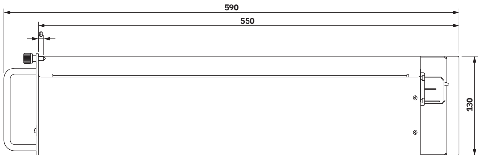
Dimensional drawing
