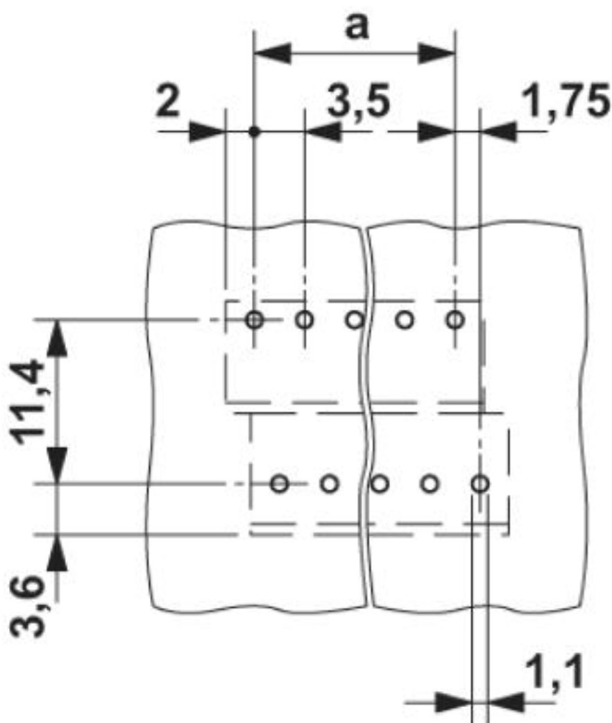
Drilling diagram
