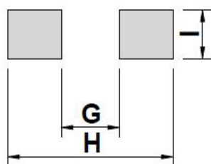
PCB PATTERN
