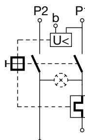
Mechanical lock-out latch
