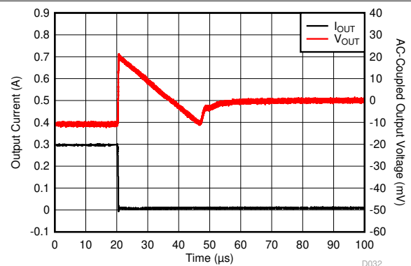
Figure 5-52. Load Transient
