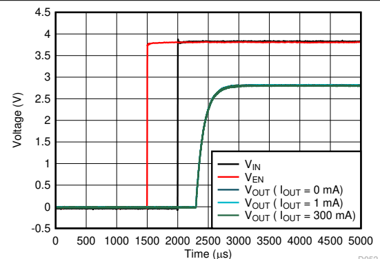
Figure 5-76. Start-Up
