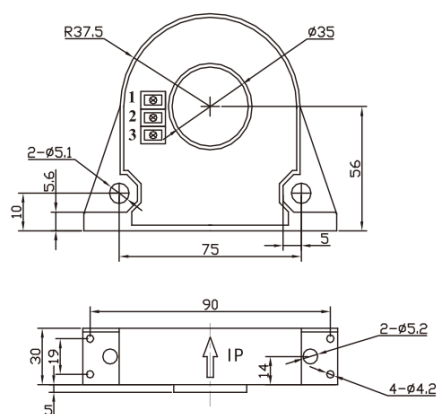
外形尺寸(mm)/Dimensions of drawing(mm)
