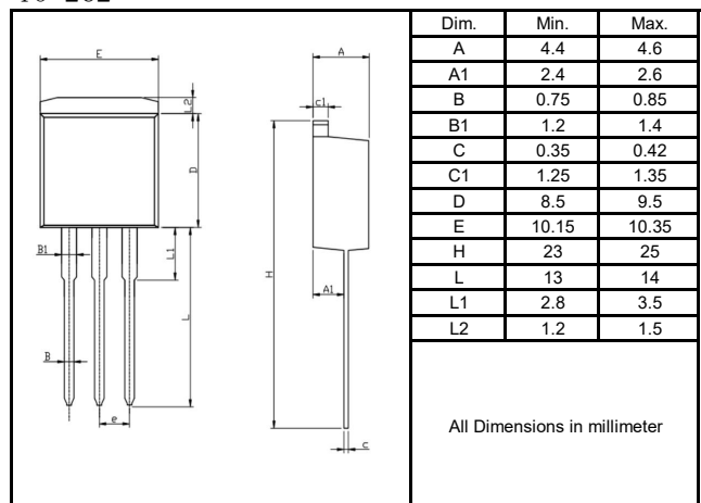
T0-262
