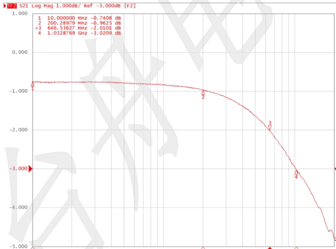
Fig.1 Switch Bandwidth or Insertion Loss
