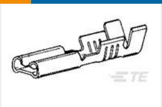
TE Part #160772-3 110 FASTON,REC.,26-22 AWG,TPBR
