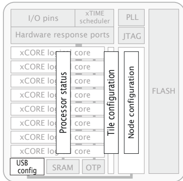
Figure 30: Registers
