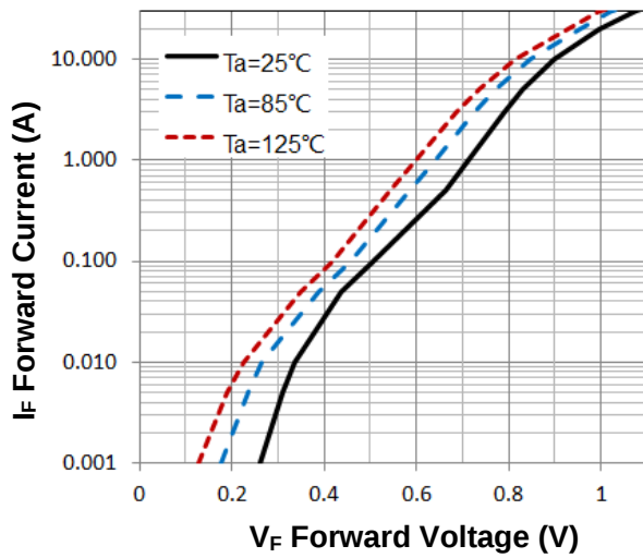
Figure 1. Forward Characteristic(typ.)
