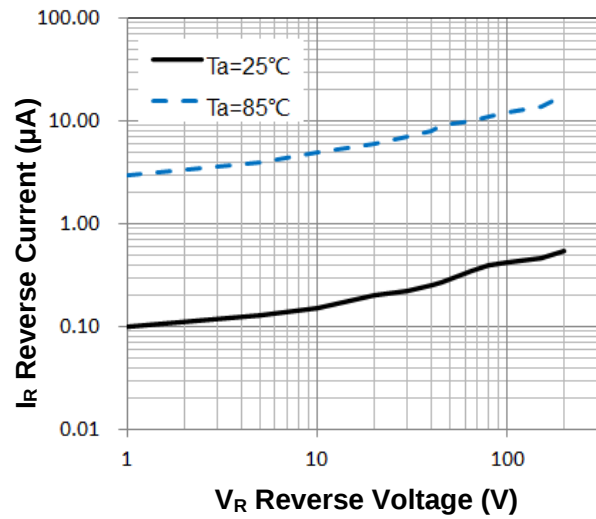
Figure 2. Reverse Characteristic (typ.)
