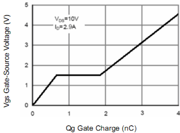
Figure 11 Gate Charge
