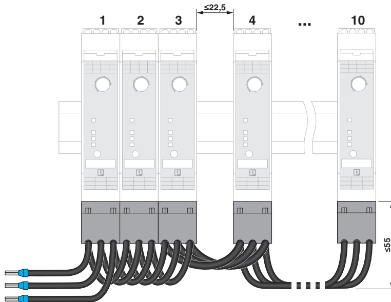
Application drawing
