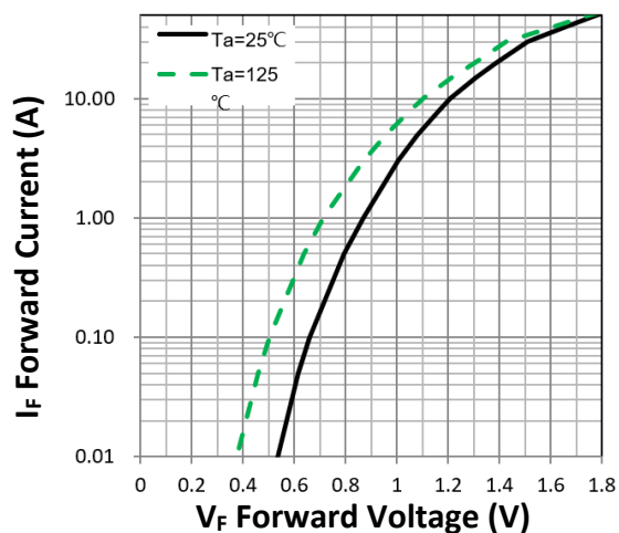
Figure 1. Forward Characteristic(typ.)
