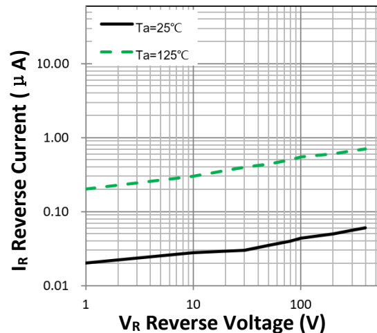
Figure 2. Reverse Characteristic (typ.)
