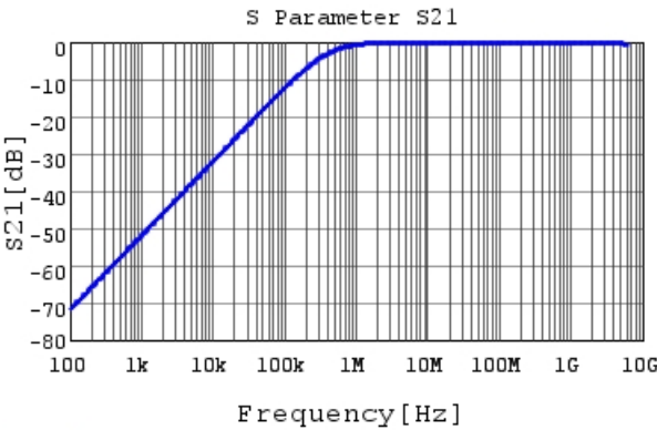
GCJ188R72A392KA01 S21 DC0V,25degC
