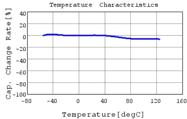
GCJ188R72A392KA01 C-Temp. capchange, DC0.0V,
