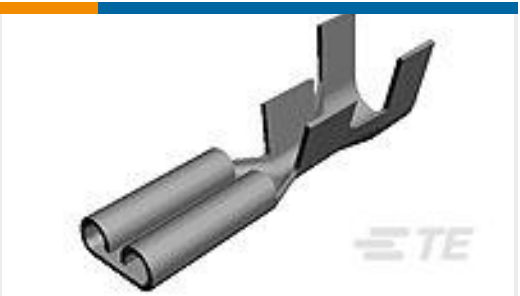
TE Part #140716-2 110 FASTON, REC., 24-22 AWG, PTBR
