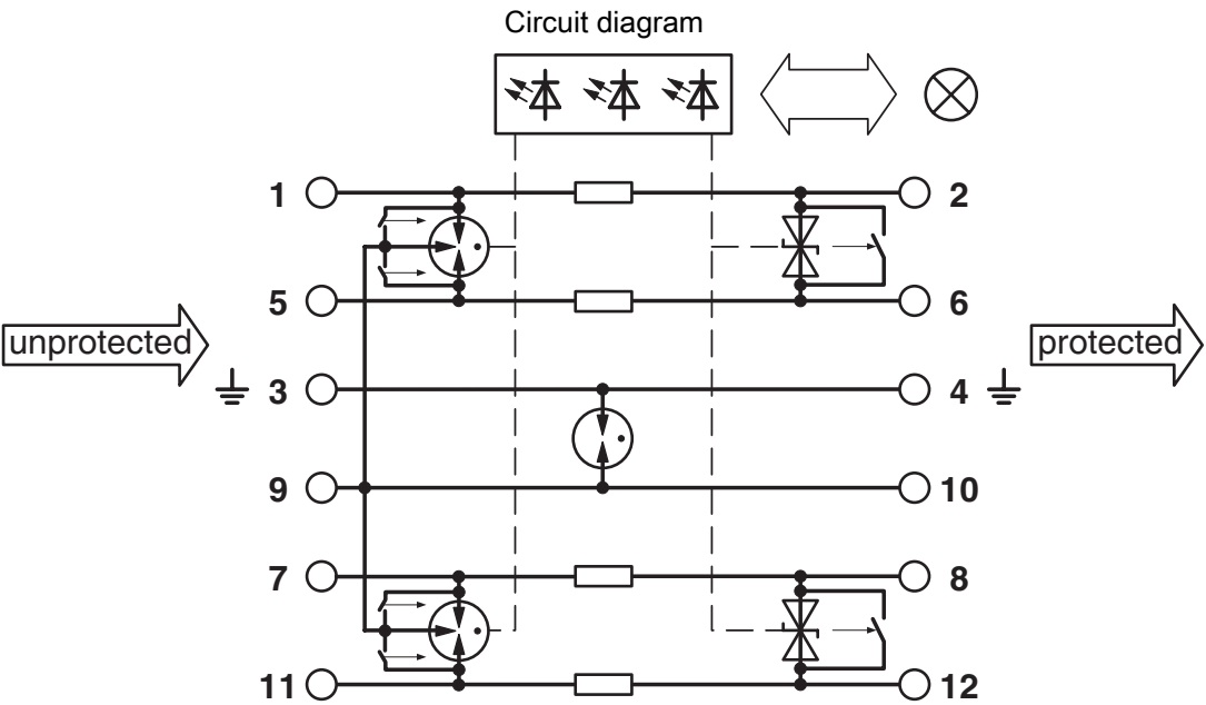
Schematic diagram
