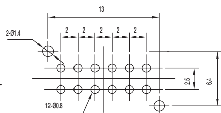
PIERCING PLAN
