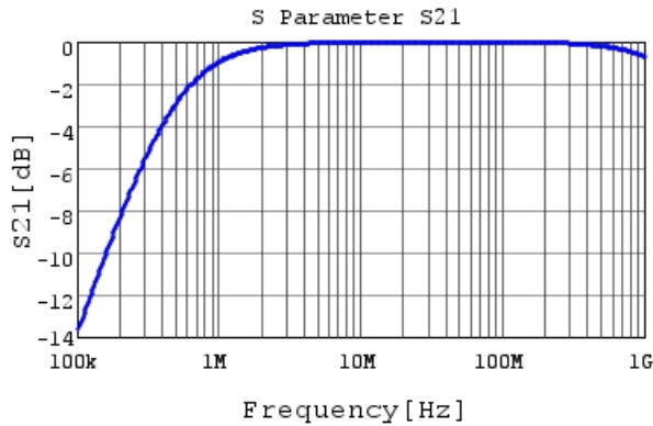
RHEL82A332K0M1H03A S21 DCOV, 25degC
