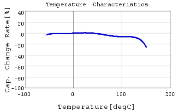
RHEL82A332K0M1H03A C-Temp. capchange, DCOV,
