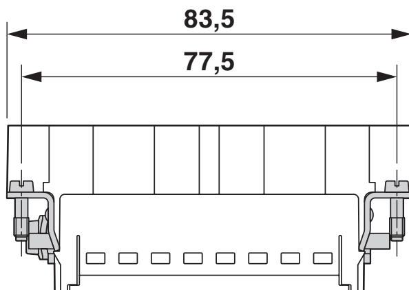
Dimensional drawing
