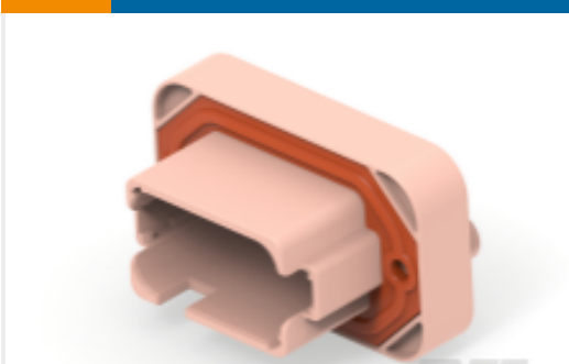
TE Part #DT13-12PD-B016 HDR, 12P, BRN, RA, ENH KEY, NI/CU, D
