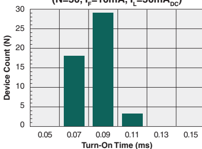
Typical Turn-On Time (N=50, I_F=10mA , I_L=50mA_{DC} )
