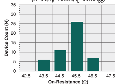
Typical On-Resistance Distribution (N=50, I_F=10mA , I_L=50mA_{DC} )
