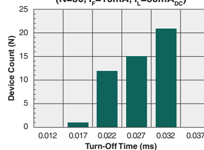
Typical Turn-Off Time (N=50, I_F=10mA , I_L=50mA_{DC} )
