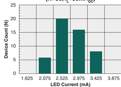
Typical I_F for Switch Operation (N=50, I_L=50mA_{DC} )
