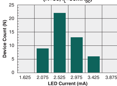
Typical I_F for Switch Dropout (N=50, I_L=50mA_{DC} )
