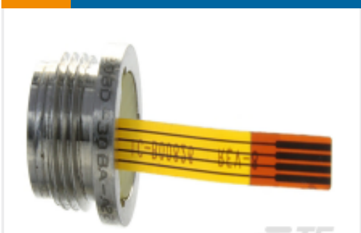
TE Part #89BSD-028BA-A 28 BARA 316L DIGITAL PRESSURE SENSOR
