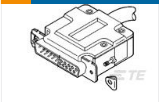
TE Part #5207908-4 STRAIN REL W/SCREW RET KIT
