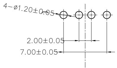
FRONT EDGE OF CONNECTOR PCB LAYOUT
