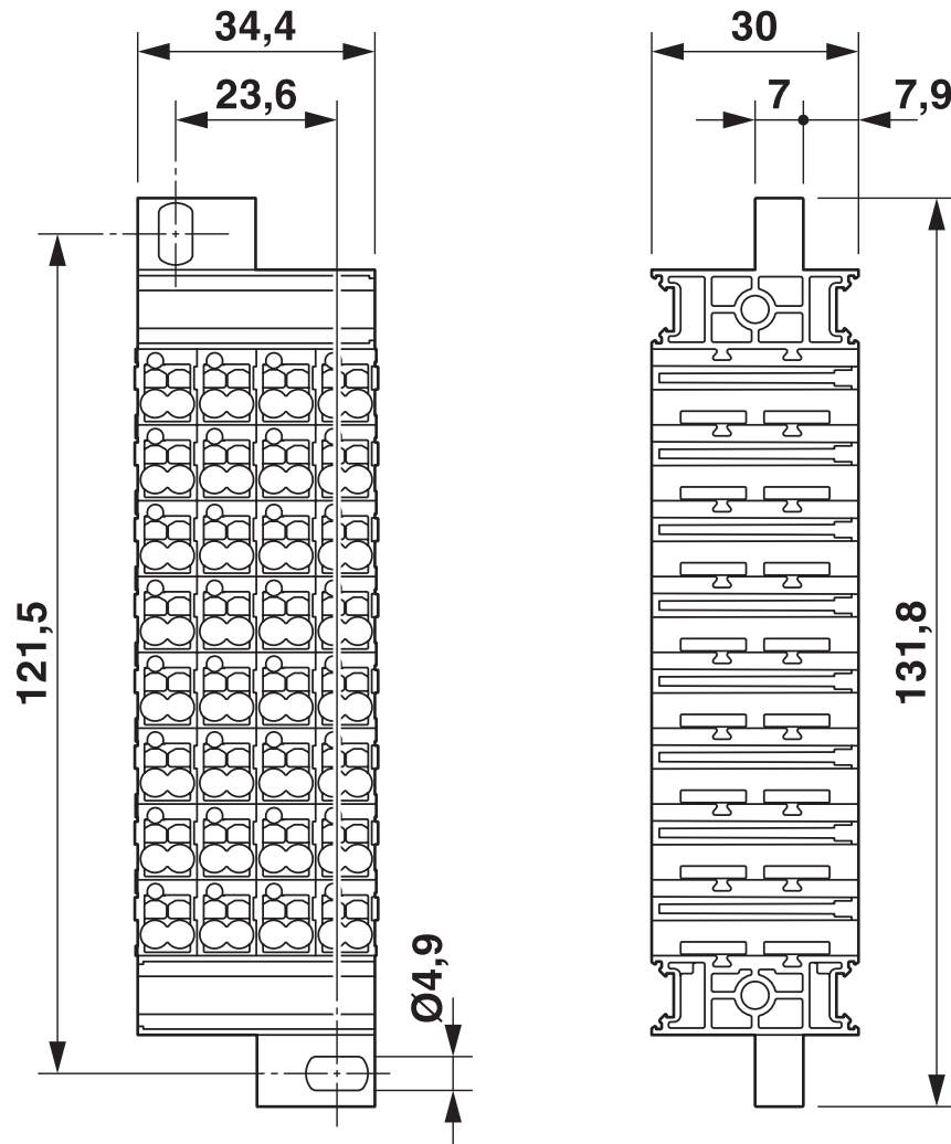
Dimensional drawing
