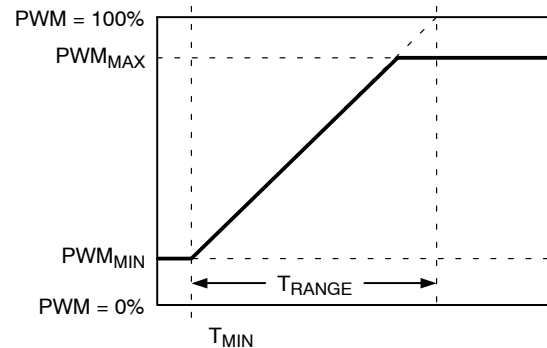
Figure 46. T RANGE
