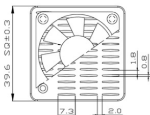
FHE40-40-xx
