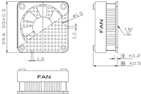
FHP40-40-xx
