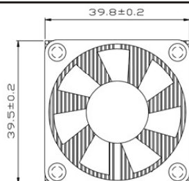
FHL40-40-xx
