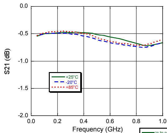
Insertion Loss to 1 GHz (power off)
