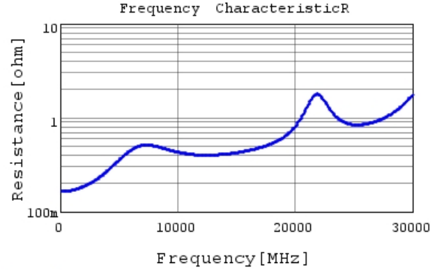
GRM0115C1E4R2BE01 R DCOV,25degC
