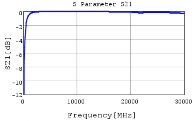
GRM0115C1E4R2BE01 S21 DCOV, 25degC
