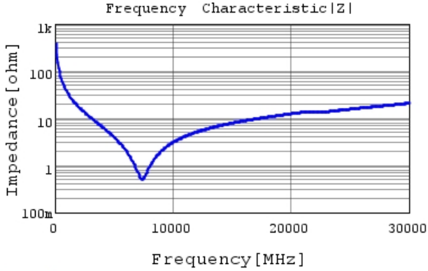
GRM0115C1E4R2BE01 |Z| DCOV,25degC
