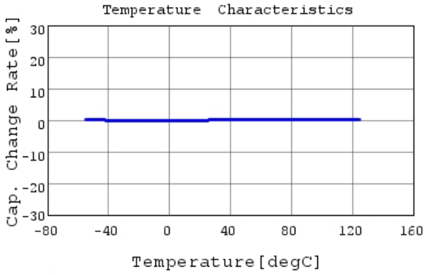
GRM0115C1E4R2BE01 C-Temp. capchange, DCOV, 1
