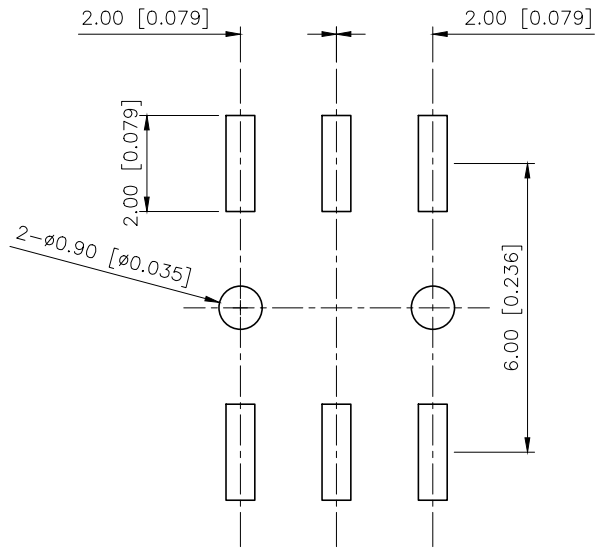
PCB LAYOUT
