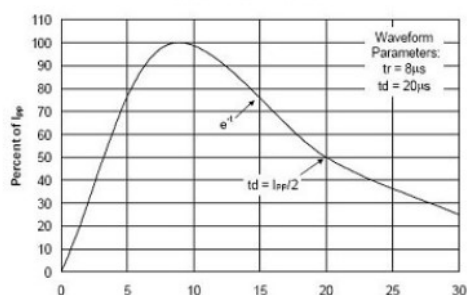
Pulse Waveform
