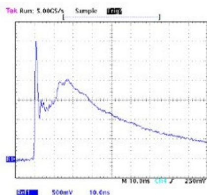
Pulse Waveform
