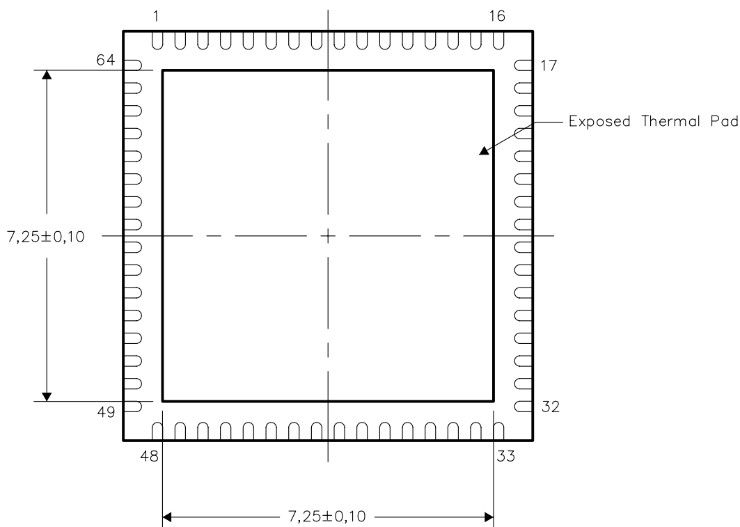
Bottom View
