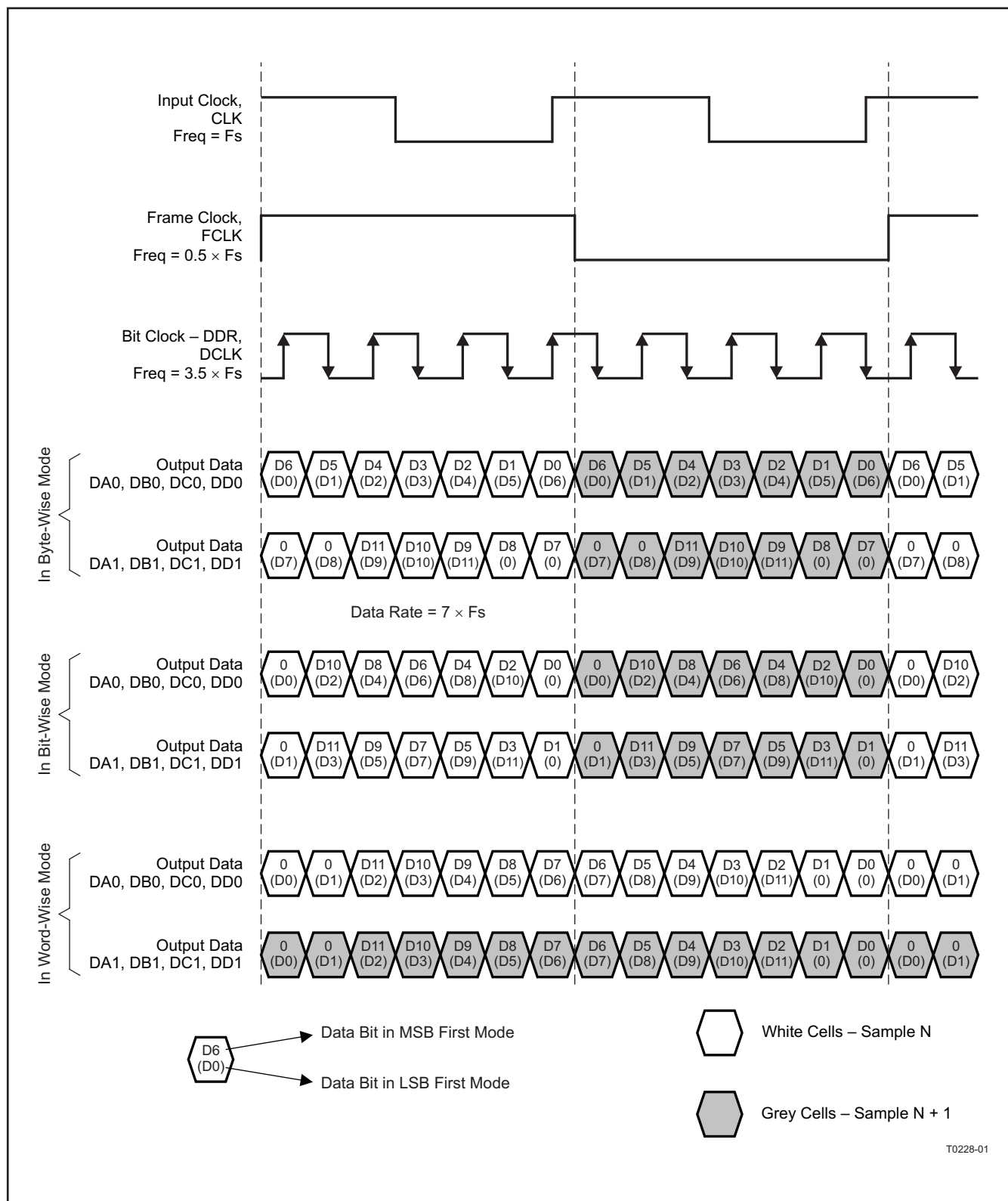
Figure 78. 2-Wire interface 14× Serialization - DDR Bit Clock
