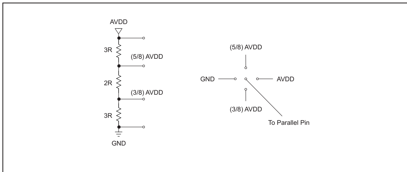
Figure 3. Simple Scheme to Configure Parallel Pins
