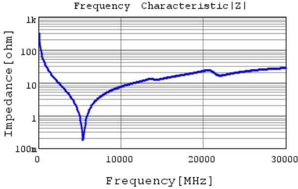
GJM0225C1C5R3BB01 |Z| DCOV, 25degC
