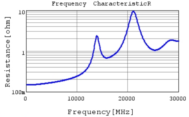
GJM0225C1C5R3BB01 R DCOV, 25degC
