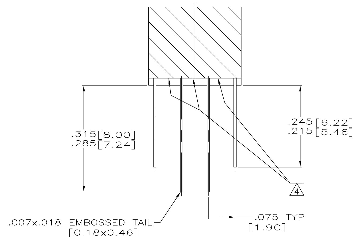
SECTION T-T SCALE 8:1
